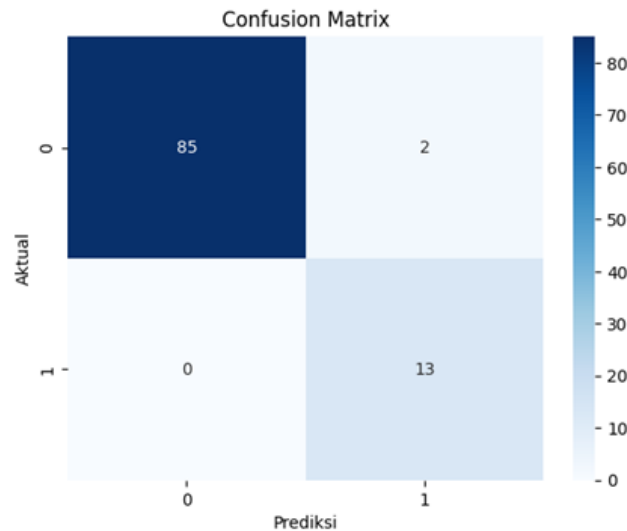
Gambar 2. Confusion Matriks
